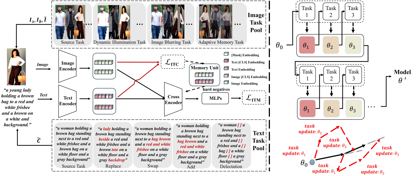
Fig. 2. Overview of the proposed domain-agnostic pretraining on the synthetic dataset, i.e. , MALS. (1) We initially design stylized image tasks involving dynamic illumination, image blurring and adaptive memory, while we apply text augmentation to simulate the real-world natural language inputs. Then augmented image-text pairs are fed into the encoders, and calculate the image-text contrastive loss (ITC) and image-text matching loss (ITM). (2) Subsequently, guided by the meta-learning strategy, model parameters are optimized through gradient updates directed by the loss function, adapting to diverse task requirements. The red dashed line represents the task-specific updates, reflecting the model’s rapid optimization in specific tasks (lines 6-10 in Alg.1). The gray dashed line represents the fast update, which helps the model quickly adapt to new tasks by adjusting global parameters (line 14 in Alg.1). The black line represents the slow update, ensuring gradual convergence through global optimization (line 17 in Alg.1).
