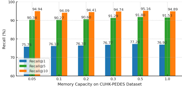
Fig. 4. Ablation Study on the memory capacity in our CAMEL. We apply 5%, 10%, 20%, 30%, 50% and 100% data pairs to pre-train, and then report the fine-tuned performance on CUHK-PEDES dataset. The percentage refers to the current capacity relative to the sample size extracted for dynamic illumination and blurring tasks.
