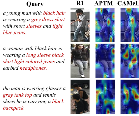
Fig. 7. Visual comparison of cross attention maps generated by the APTM [14] and Ours (CAMEL) using Grad-CAM [91]. We could observe that the regions highlighted by the proposed methodology exhibit significant alignment with the keywords used in the query sentences, indicating effective matching performance.
